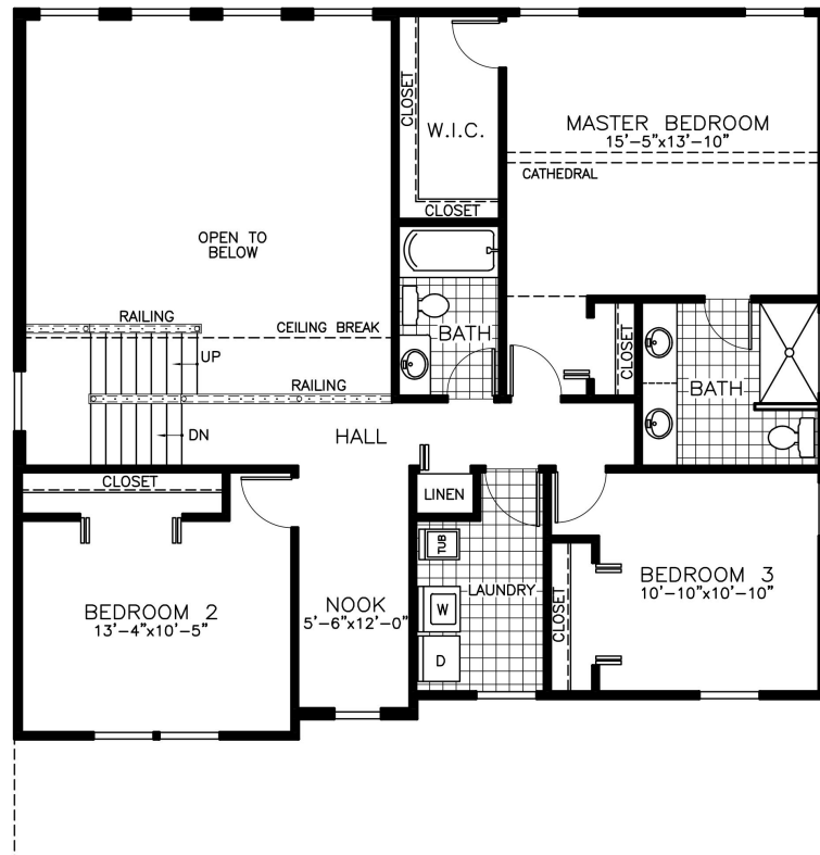
Second Floor with Nook above Foyer Option Adds 48 sq. ft.
