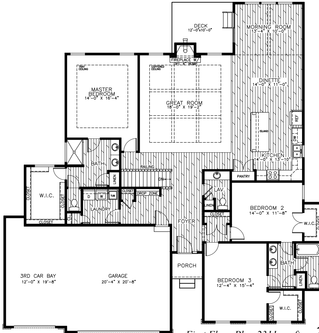
First Floor Plan 2311 sq. ft.
